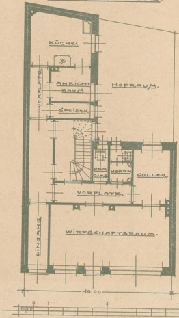
ERDGESCHOSS.
